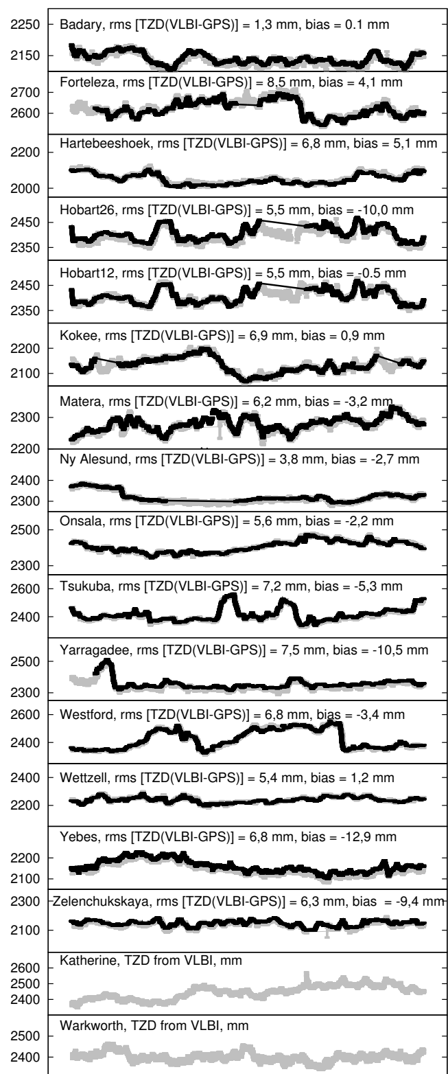
Fig. 2 TZD intra-day (VLBI compared with GPS) variations from CONT14.
